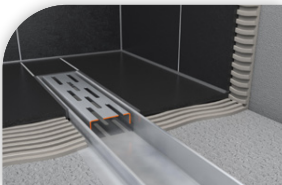
Easydrain doorsnee
